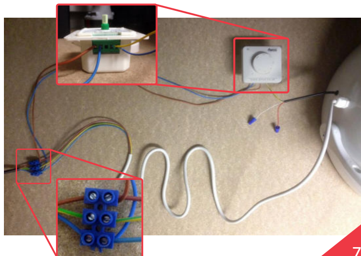
SPEED CONTROL DIAL
